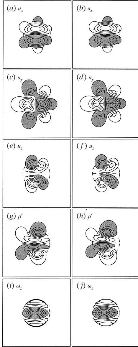
FIGURE 11. Comparison between the numerical (left-hand panels) and theoretical (right-hand panels) eigenmodes given by (5.5)–(5.7) for F_h = 0.033 , k_z = 8.25 and \{Re = 10000, Sc = 1\} . (a, b) u_x ; (c, d) u_y ; (e, f) u_z ; (g, h) \rho' ; (i, j) \omega_z . The contour interval is not the same for each variable but is identical for the theoretical and numerical contour maps: 0.725 for u_x , 0.34 for u_y , 0.0238 for u_z , 4.47 for \rho' and 3.32 for \omega_z . Only a domain of size 5 \times 5 is represented while the original computational domain is 9 \times 9 . For other details refer to the legend of figure 4.
